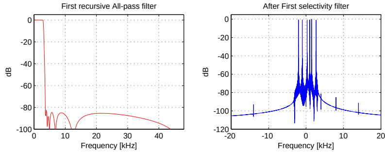
Figure 16: The left figure show the spectrum of the recursive All-pass selectivity filter, and the right the output.
