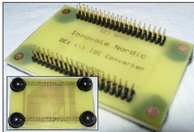
Figure 3: Photograph of IDE to DE1 converter
