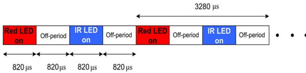
Figure 3. LED controlling scheme
