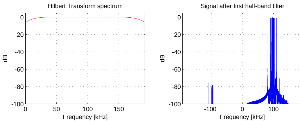
Figure 12: Left figure show the spectrum of the Hilbert transform, and the rigth the output since the Hilbert transform, where the negative frequency are not completely zeroed out but attenuated 80 dB.
