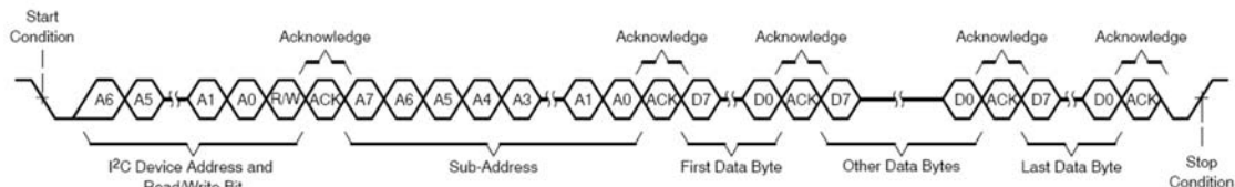
Figure 12: Multiple byte write transfer (from TI datasheet TAS5504)
