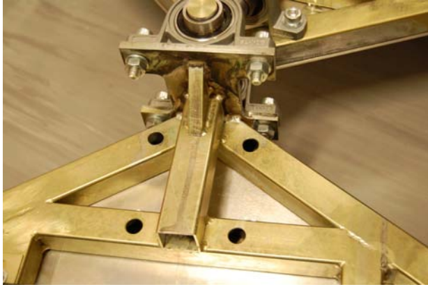
Figur 9, Midjoint welding
