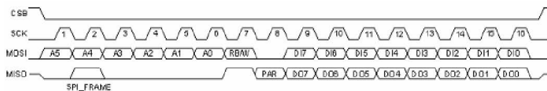
Figure 2. 4-wire SPI protocol in VTI3000-E04 accelerometer
