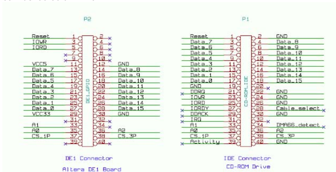
Figure 4: Schematic of IDE to DE1 converter
