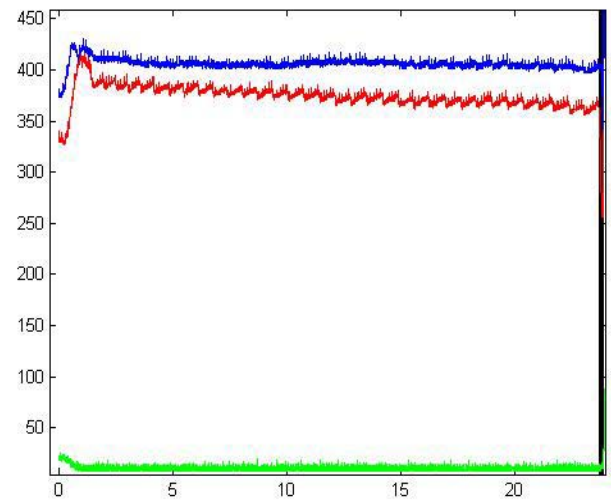
Figure 4b. Measurements from the pulse oximeter (red LED = red, IR-LED = blue, both LEDs off = green)
