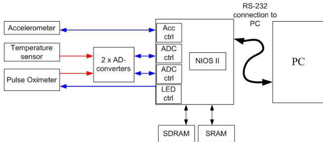
Figure 1. Block diagram of the measurement system
