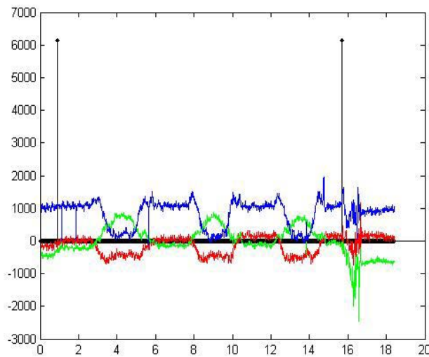
Figure 4a. Measurements from the accelerometer ( x-axis = red, y-axis = green, z-axis = blue)
